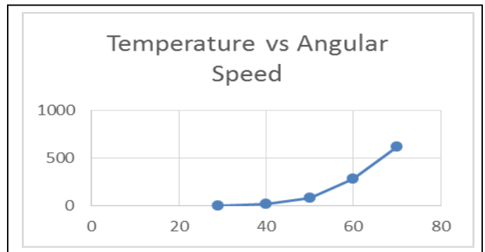
Fig. 7. Temperature in air column – Angular speed of shaft.
