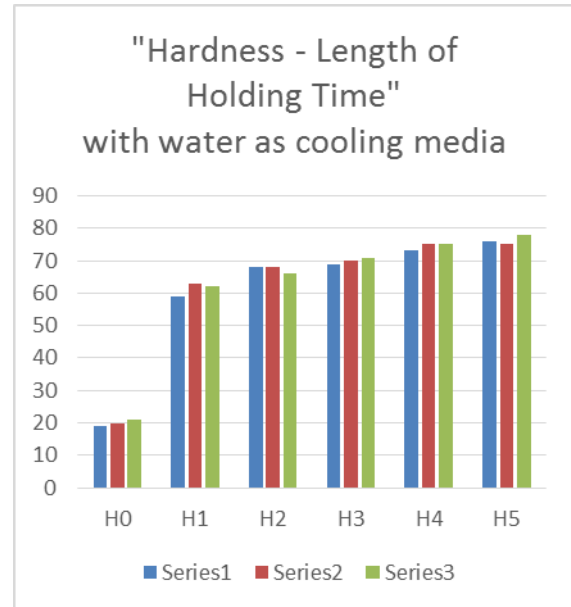
Fig. 2. Hardness – Length Of Holding Time With Water As Cooling Media.
